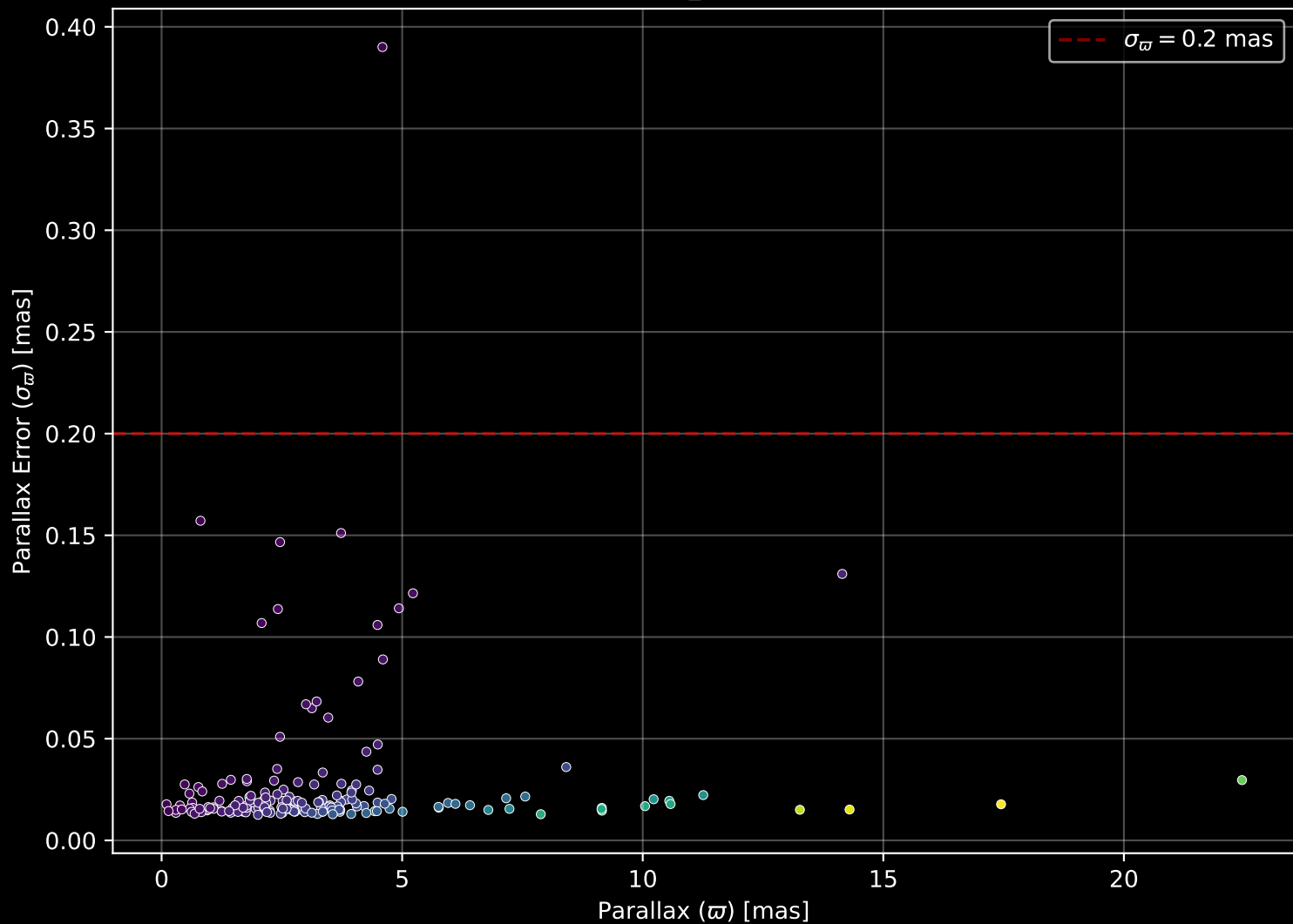
APOGEE DR17 Field: [178+44_MGA] Parallax Quality (n= 179)
