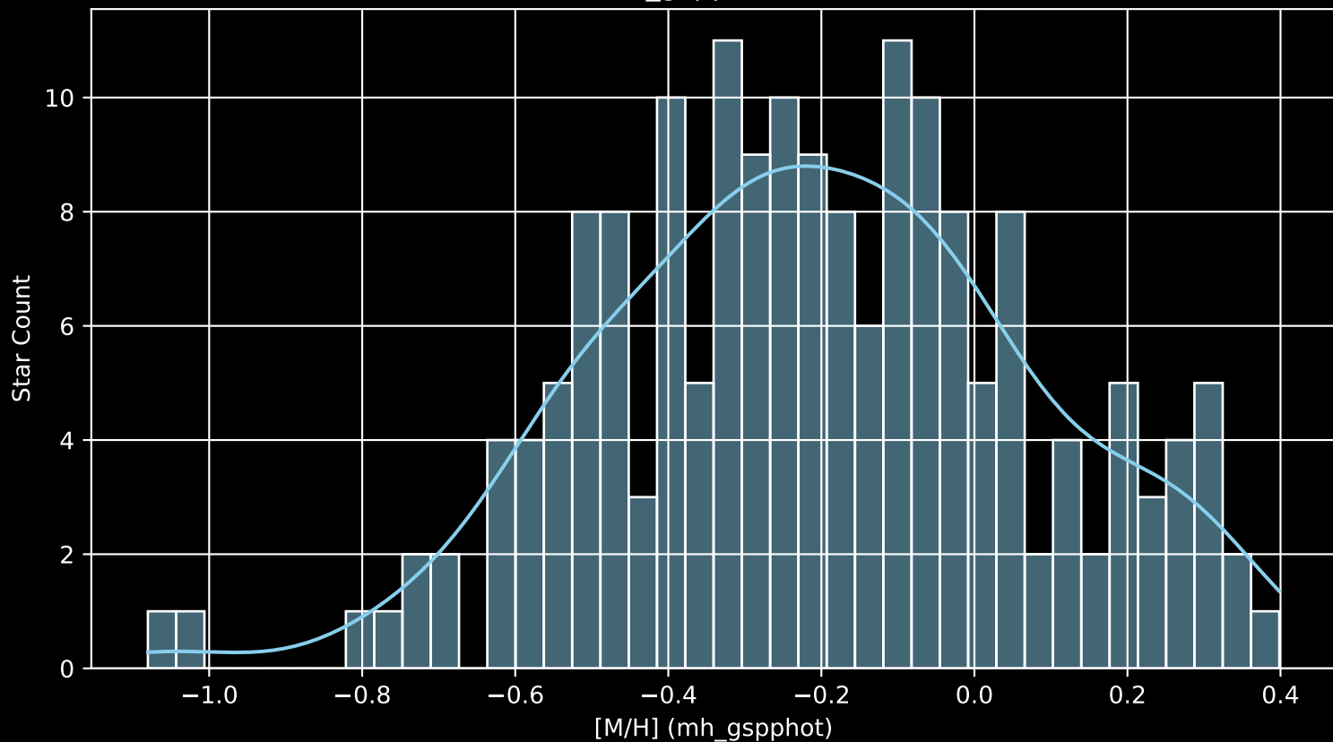
APOGEE DR17 Field: [178+44_MGA [M/H] (mh_gspphot) (n= 178)
