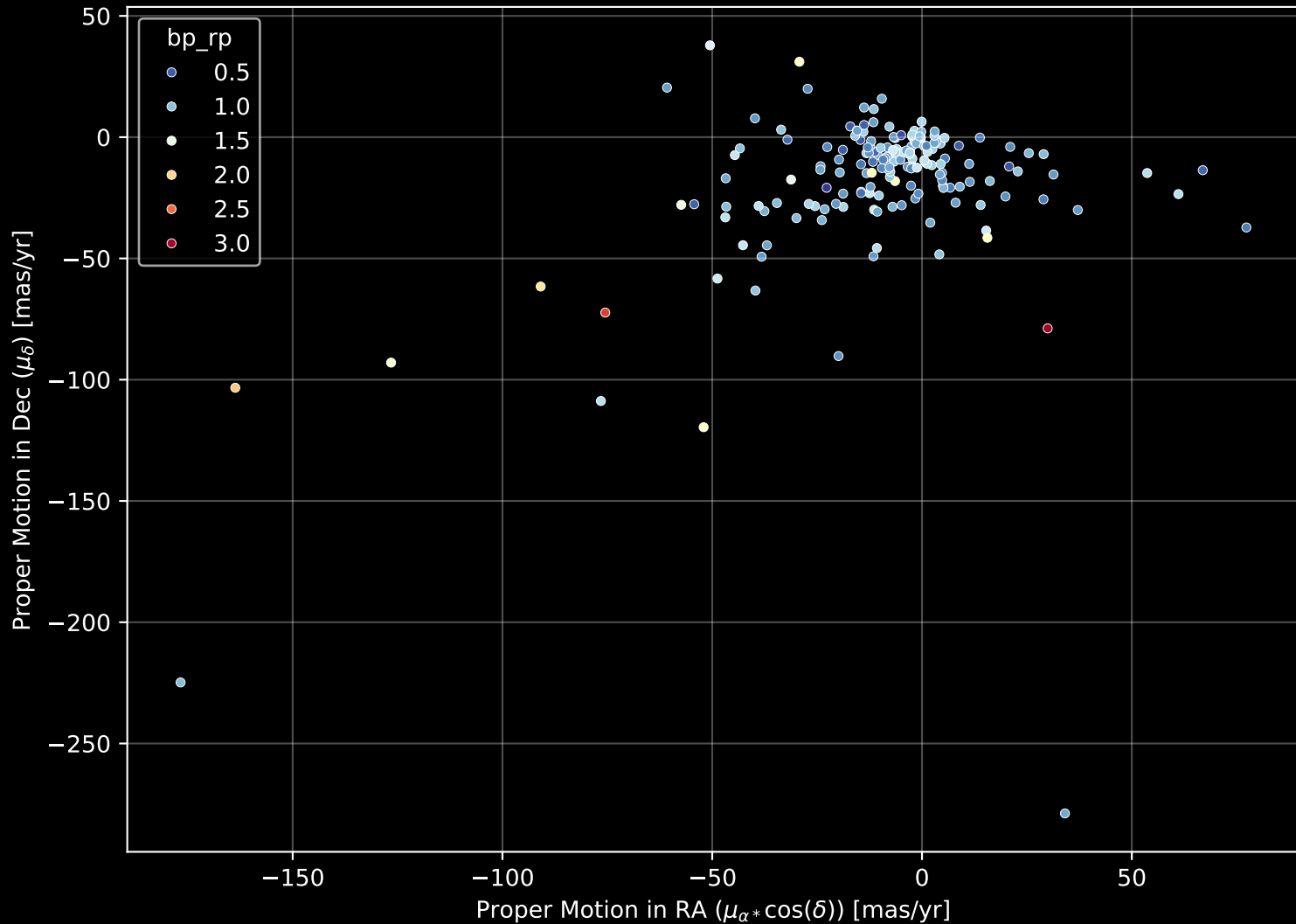
APOGEE DR17 Field: [178+44_MGA] Proper Motion Diagram (n= 179)
