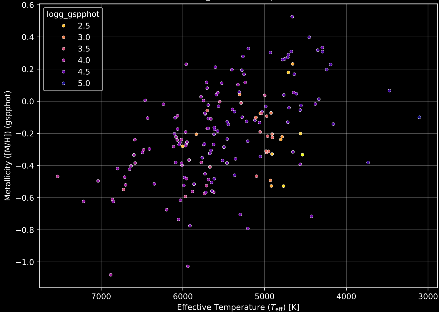
APOGEE DR17 Field: [178+44_MGA] Stellar Population Parameters (n= 179)
