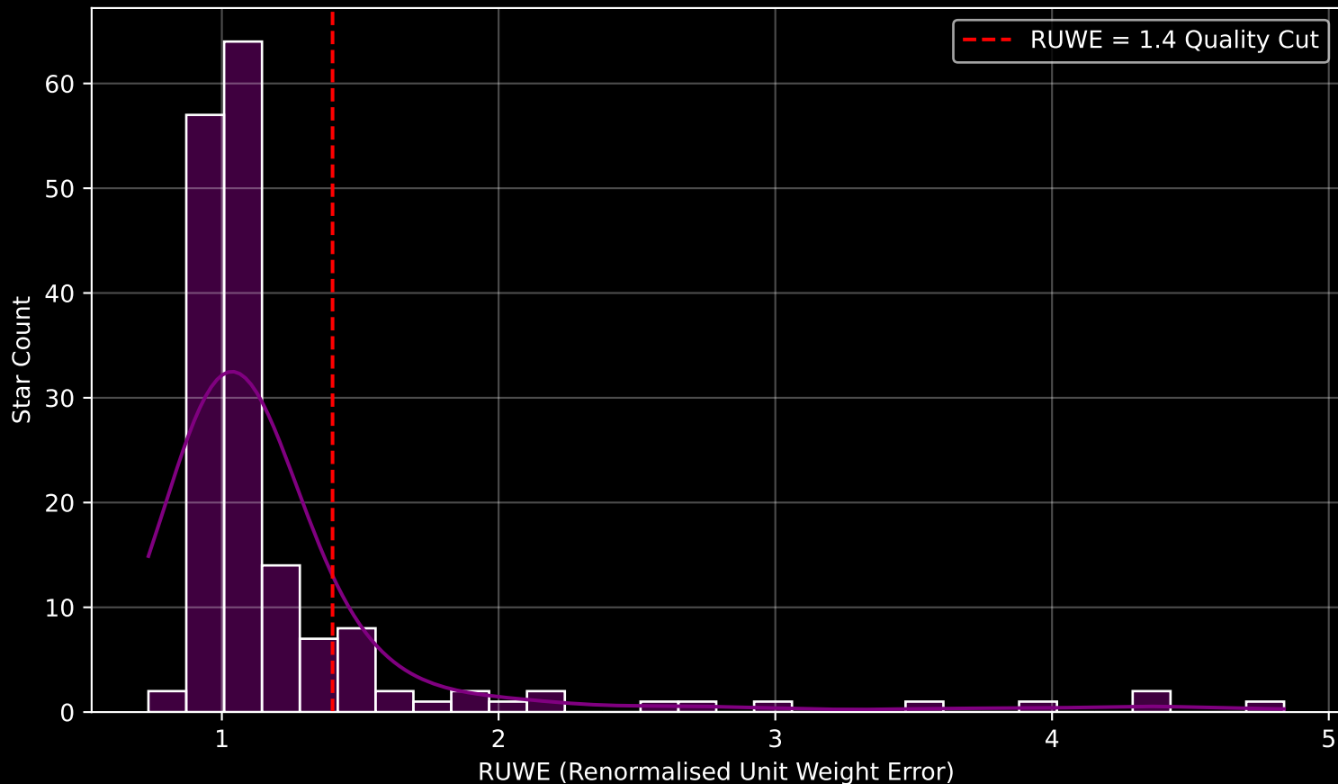
GAPOGEE DR17 Field [178+44_MGA] RUWE Distribution (n= 168)
