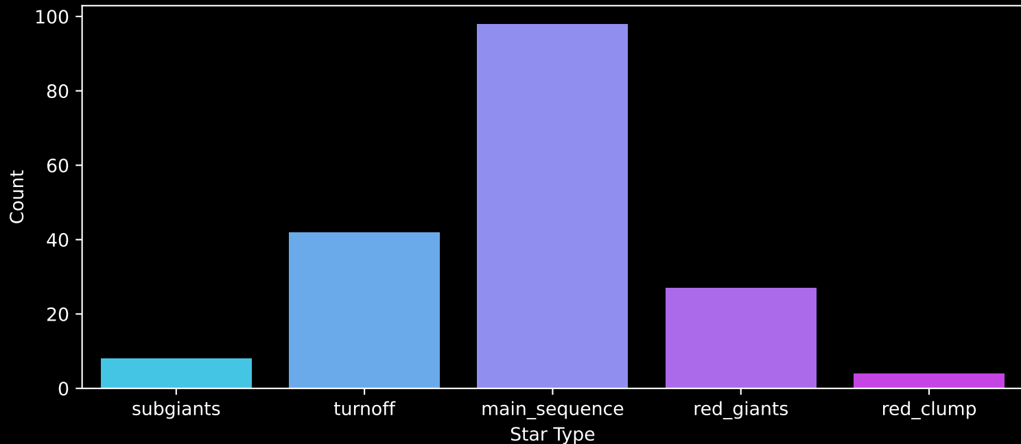
APOGEE DR17 Field: [178+44_MGA] Count plot of Star Type
